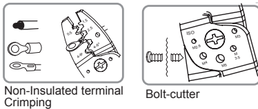
Open barrel terminal crimping
